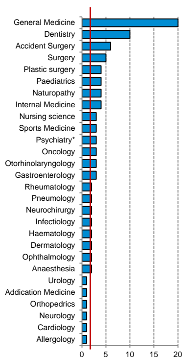
Figure 1: Number of handsearched journals in the specific medical fields (n=98). The red line indicates the median (2) of journals per field, handsearched within the last 20 years.
