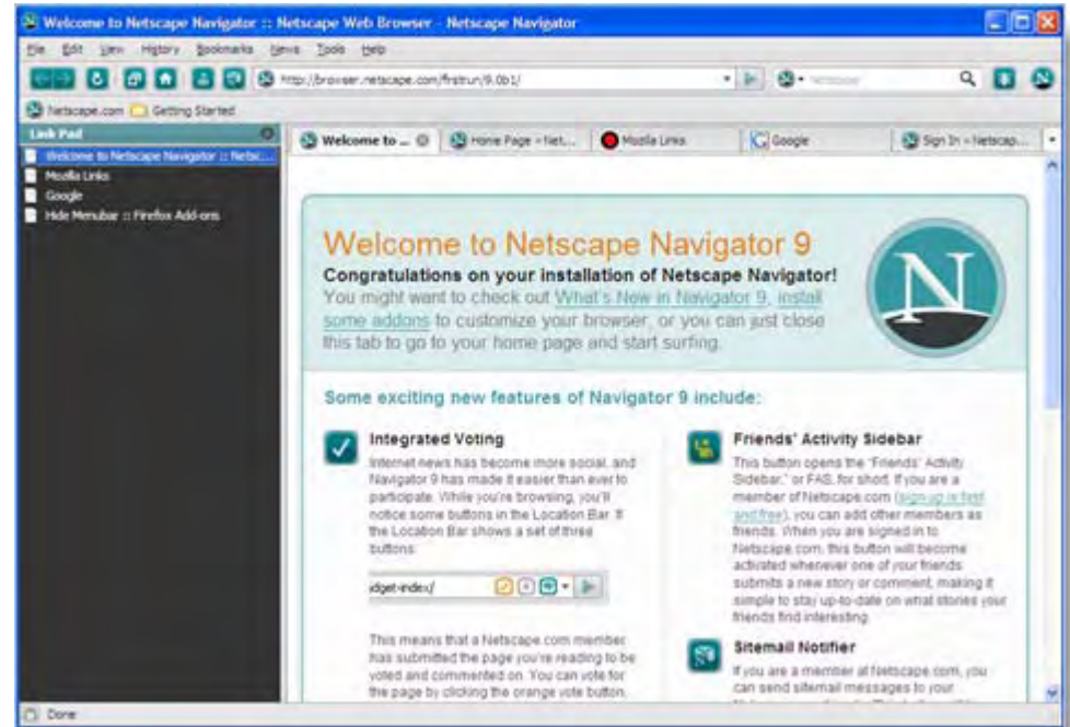
Netscape Navigator
